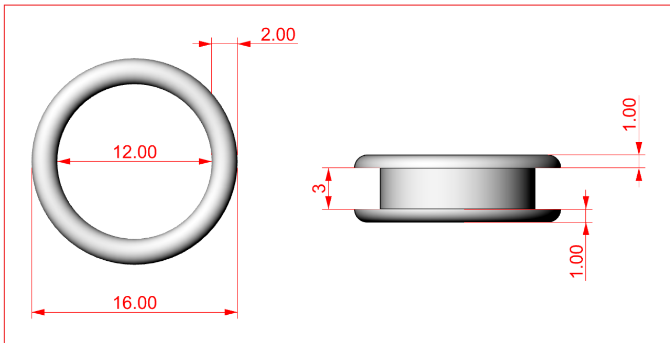
New Development: Eyelet (please see attached 3D model) x 12 pieces
