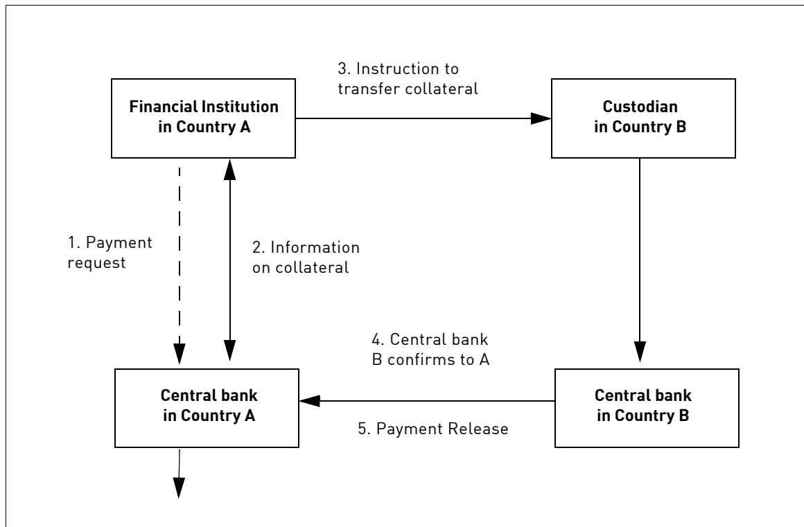
Figure 3.9 T2 RTGS
