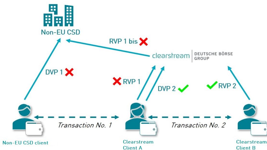
Figure 3.12 Back-to-back transaction.
